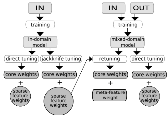
Figure 2: In-domain (IN) and mixed-domain (IN+OUT) models with three tuning schemes for tuning sparse feature weights: direct tuning, jackknife tuning and retuning.
