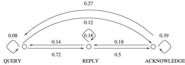
Figure 4.2: Probabilistic move bigram finite state network; not all arcs are given
