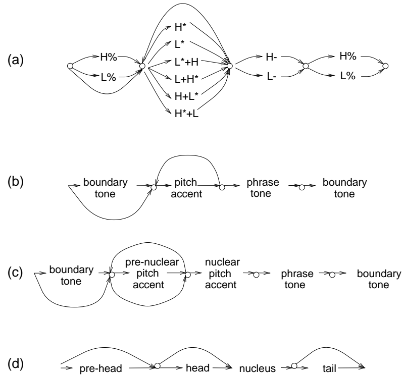
Figure 6.4: Intonation structure represented by finite state networks
