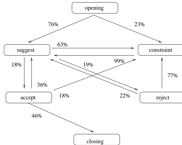
Figure 4.3: Markov model of dialogue with transitional probabilities. Source: Woszczyna and Waibel (1994)
