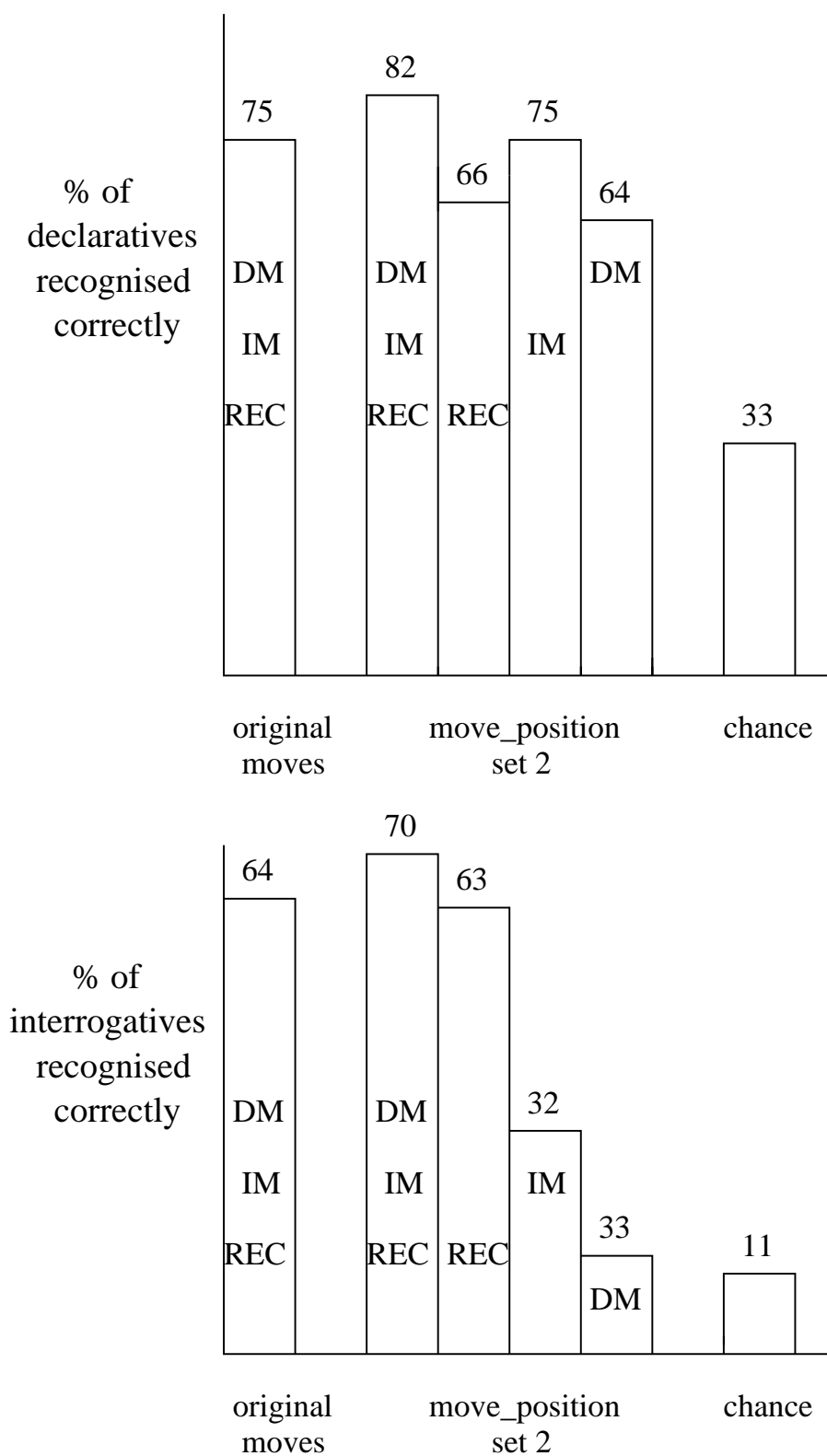
Figure 8.6: Percentage of interrogative and declarative type utterances correctly recognised
