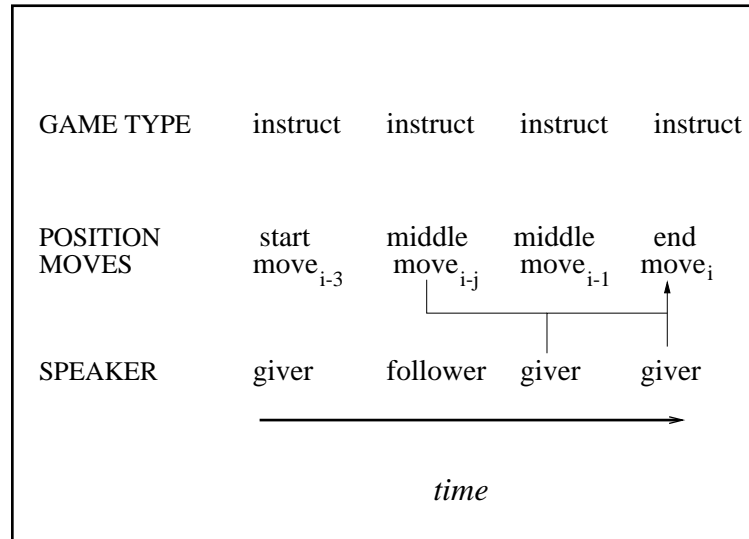
Figure 8.2: Model F for move_position modelling
