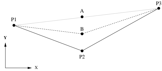
Figure 5: Smoothing.
