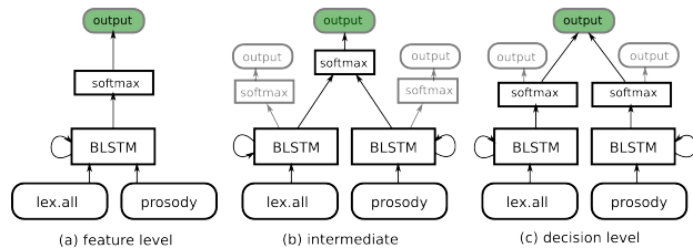
Figure 1: BLSTM feature fusion at different levels.
