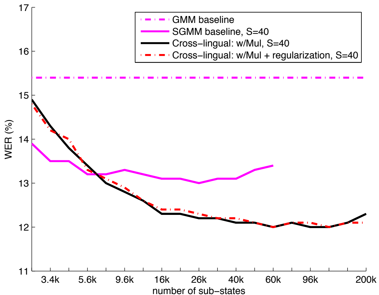
Fig. 6. WER of baseline cross-lingual systems, 15h training data, tested on the development dataset.
