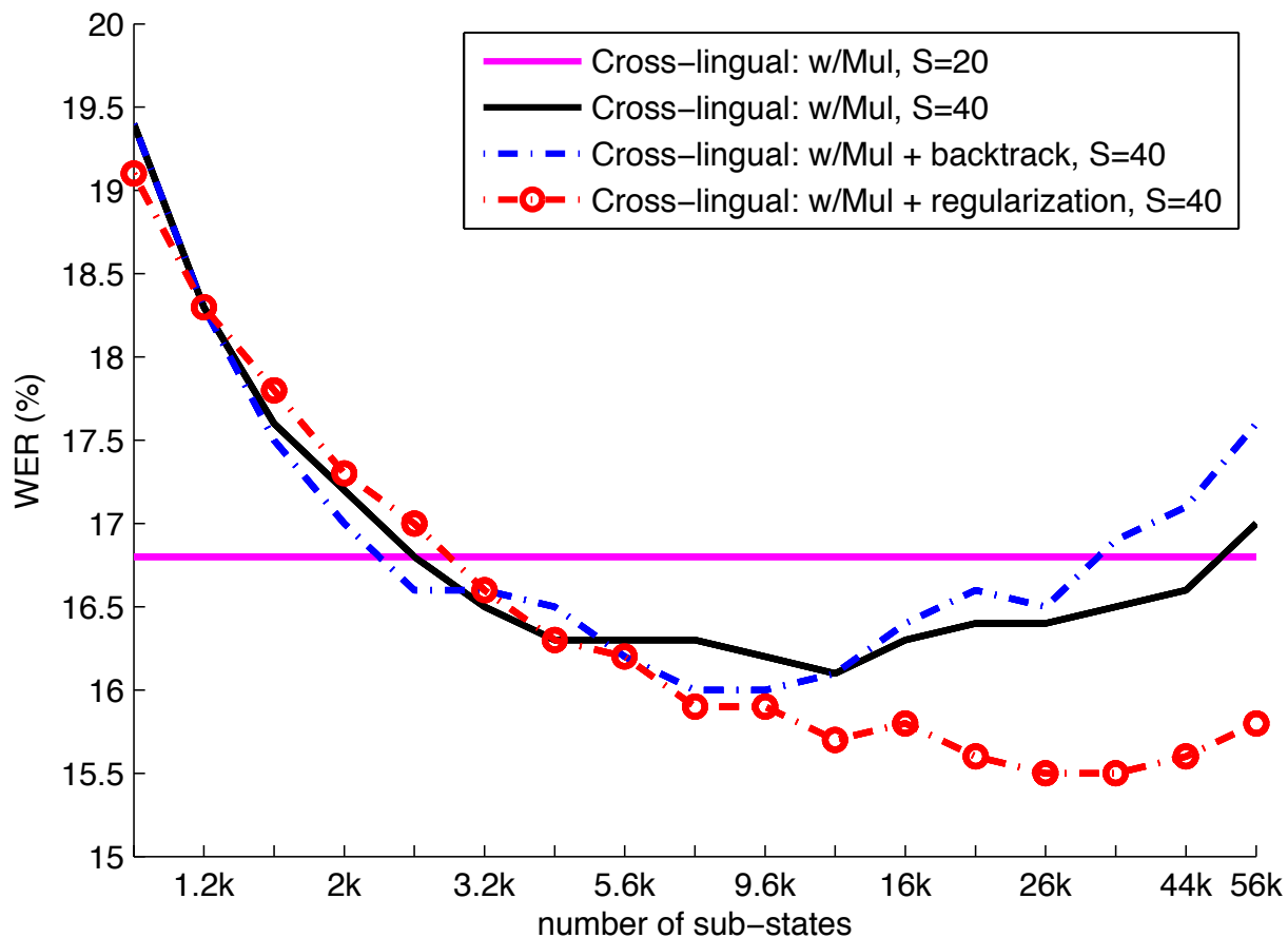
Fig. 7. WER of regularized cross-lingual systems, 1h training data, tested on the development dataset. “Cross-lingual: w/Mul, S = 20” corresponds to the best results of the same system by tuning the number of sub-states that is shown in Fig. 4.
