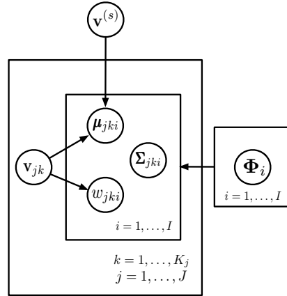
Fig. 1. Model structure of a SGMM acoustic model, with total J HMM states, and each has K_j sub-states. Each sub-state is modelled by a GMM with I components, whose parameters are derived from \Phi_i = \{\mathbf{M}_i, \mathbf{N}_i, \mathbf{w}_i, \Sigma_i\} and (\mathbf{v}_{jk}, \mathbf{v}^{(s)}) using Eq. (2) and (3), and for covariance \Sigma_{jki} = \Sigma_i .
