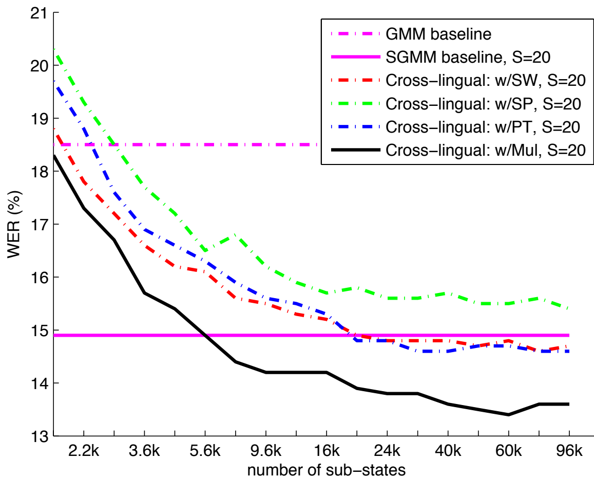
Fig. 5. WER of baseline cross-lingual systems, 5h training data, tested on the development dataset. Only the lowest WER of SGMM baseline system by tuning the number of sub-states is given for clarity.
