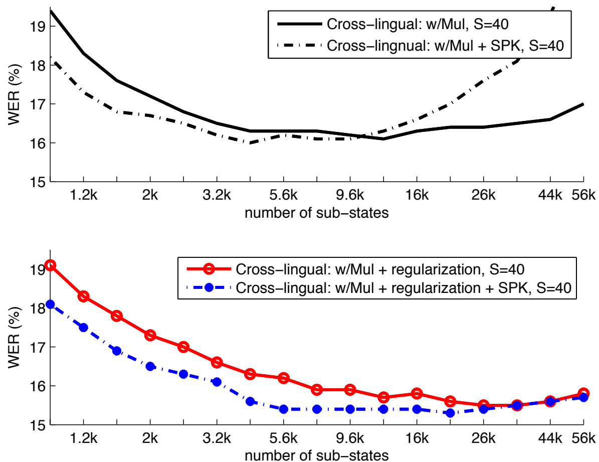
Fig. 12. WER of baseline (above) and regularized (below) cross-lingual systems using speaker subspace, 1h training data, tested on the development dataset.
