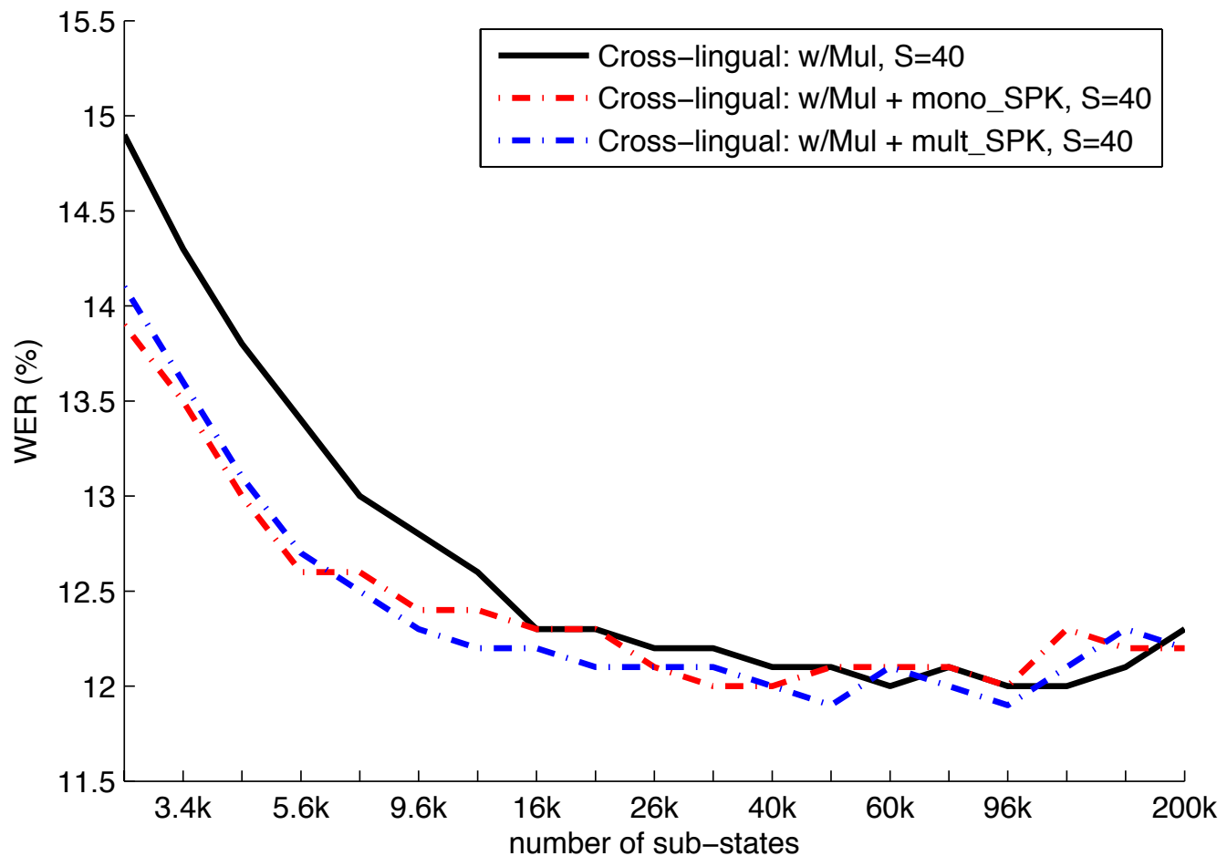
Fig. 14. WER of cross-lingual systems using speaker subspace, 15h training data, tested on the development dataset.
