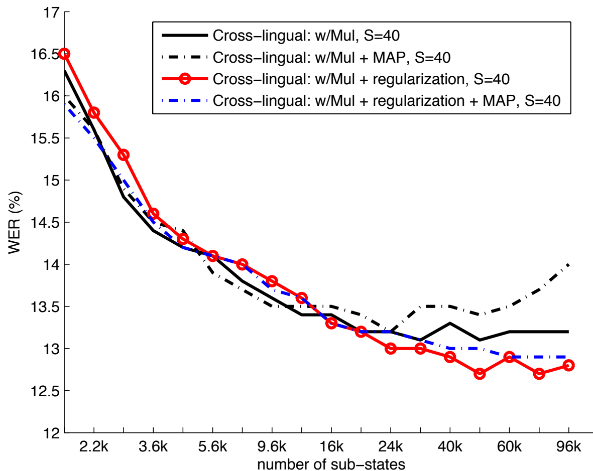
Fig. 10. WER of MAP-adapted cross-lingual systems, 5h training data, tested on the development dataset.
