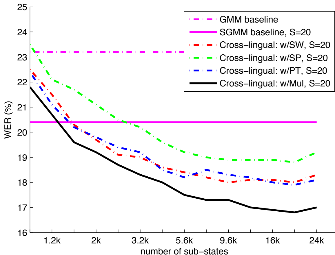
Fig. 4. WER of baseline cross-lingual systems, 1h training data, tested on the development dataset. Only the lowest WER of SGMM baseline system by tuning the number of sub-states is given for clarity.
