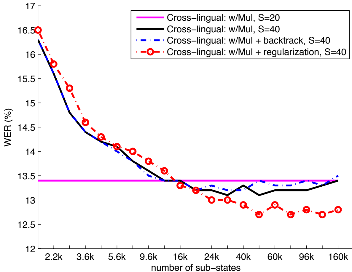
Fig. 8. WER of regularized cross-lingual systems, 5h training data, tested on the development dataset. “Cross-lingual: w/Mul, S = 20” corresponds to the best results of the same system by tuning the number of sub-states that is shown in Fig. 5.
