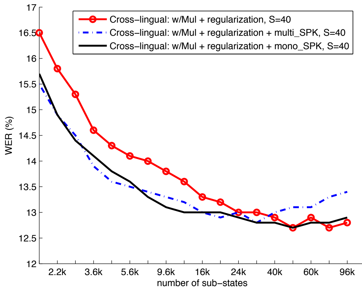
Fig. 13. WER of regularized cross-lingual systems using speaker subspace, 5h training data, tested on the development dataset.
