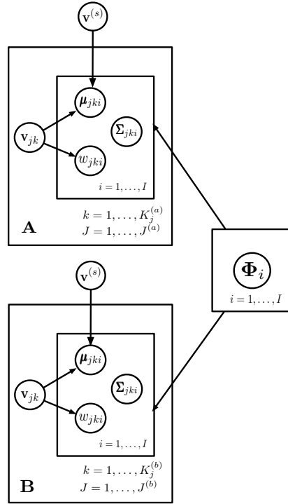
Fig. 2. An example of multilingual estimation of the globally shared parameters \Phi_i where we tie them across two source language system A and B .
