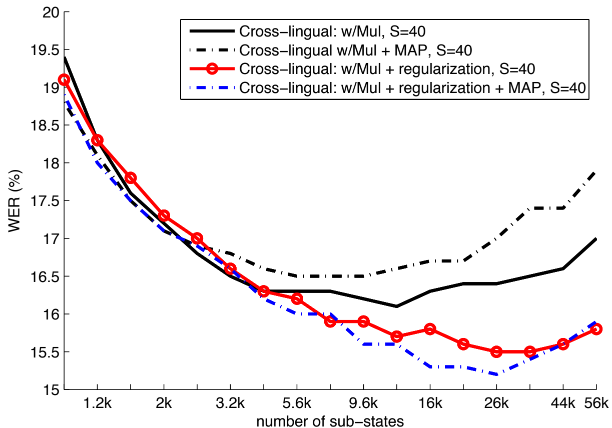
Fig. 9. WER of MAP-adapted cross-lingual systems, 1h training data, tested on the development dataset.
