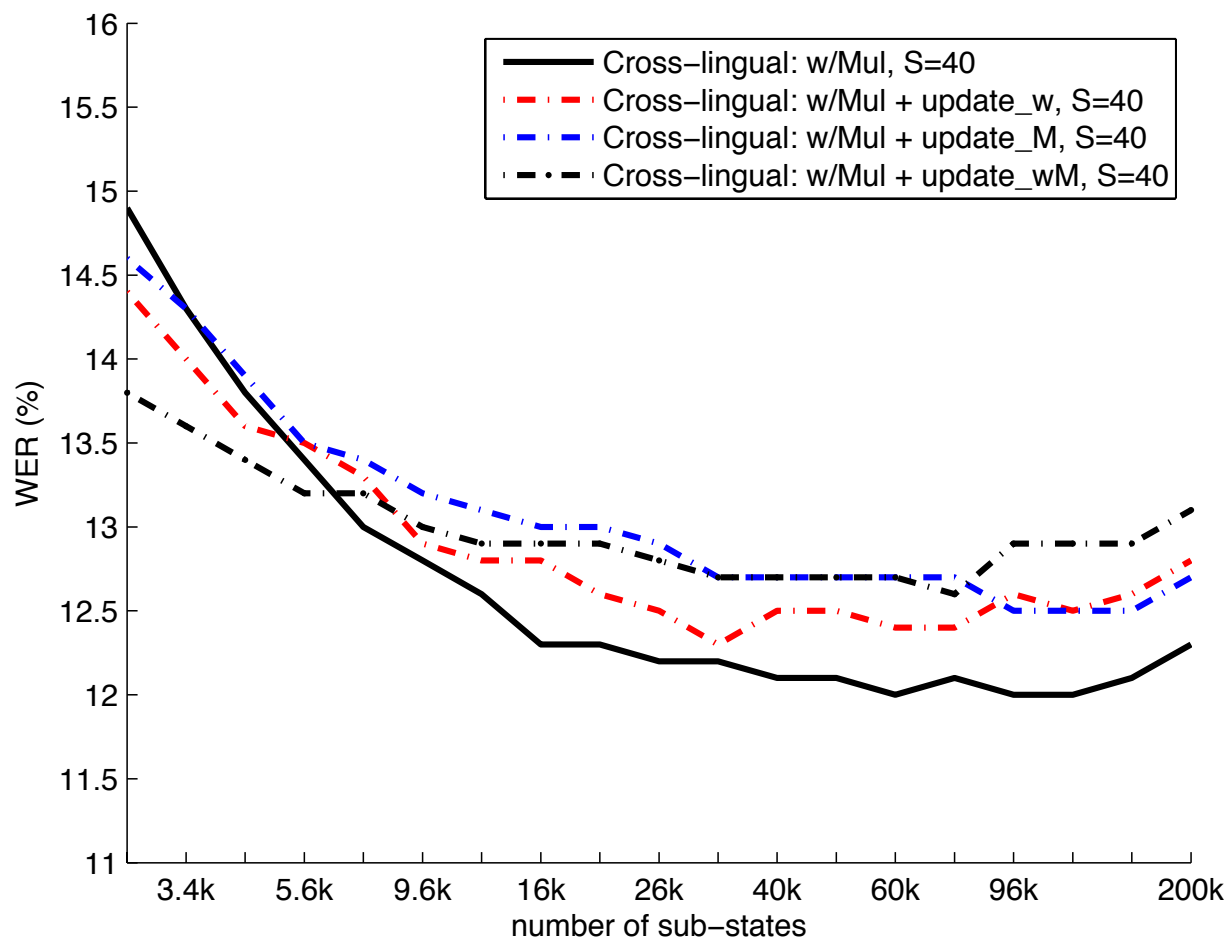
Fig. 11. WER of cross-lingual systems with global parameter update, 15h training data, tested on the development dataset.
