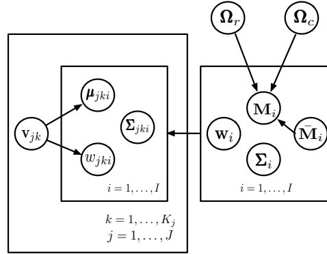
Fig. 3. MAP adaptation of \mathbf{M}_i in SGMM acoustic model. (\bar{\mathbf{M}}_i, \boldsymbol{\Omega}_r, \boldsymbol{\Omega}_c) denote the hyper-parameters of the Gaussian prior P(\mathbf{M}_i) , in which the mean \bar{\mathbf{M}}_i is indexed by I while the covariances \boldsymbol{\Omega}_r and \boldsymbol{\Omega}_c are global.
