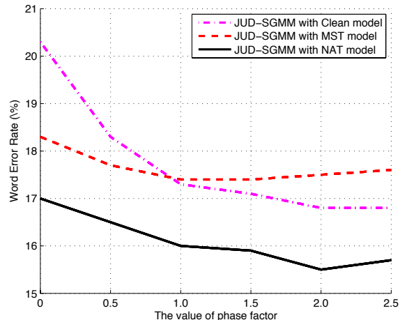
Figure 1: Results of tuning the value of phase factor \alpha in the decoding stage.
